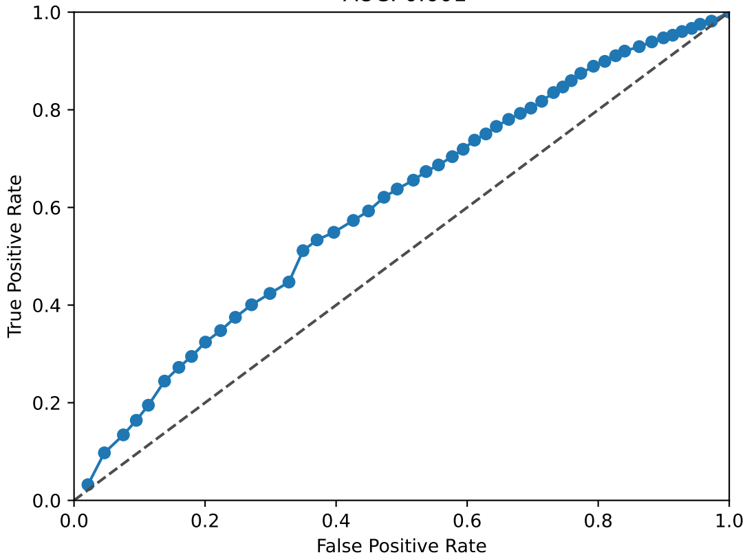
RORA_RORB ROC Curve AUC: 0.601
