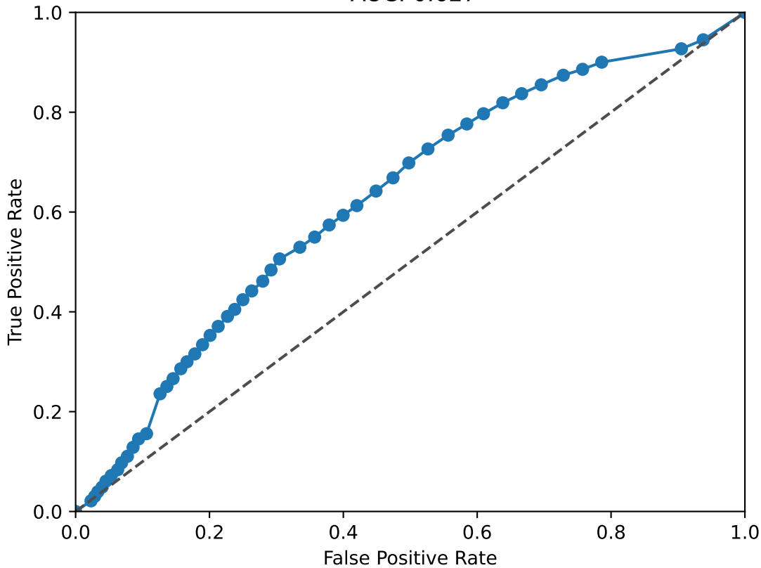
SIX1 ROC Curve AUC: 0.627
