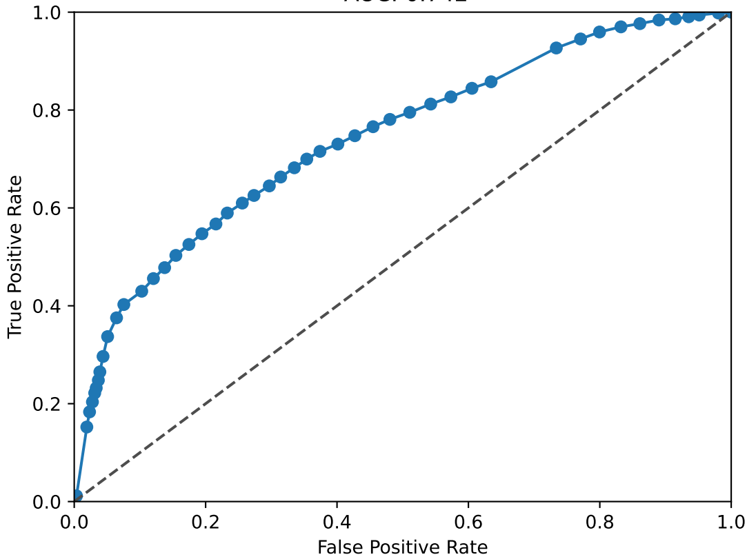
TEAD1 ROC Curve AUC: 0.742
