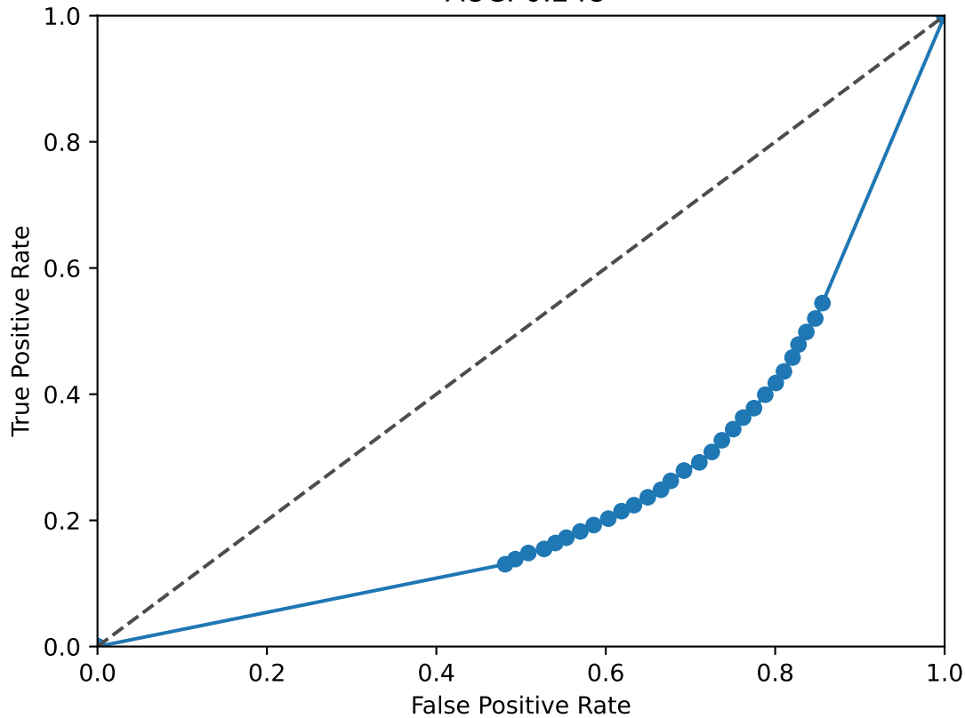
THRB ROC Curve AUC: 0.248
