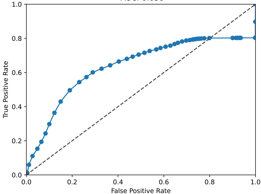
EGR1 ROC Curve AUC: 0.636
