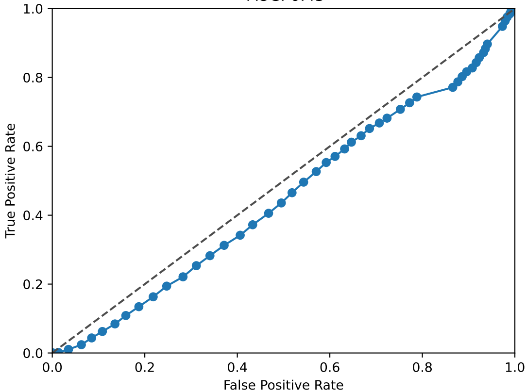
EPCAM ROC Curve AUC: 0.45
