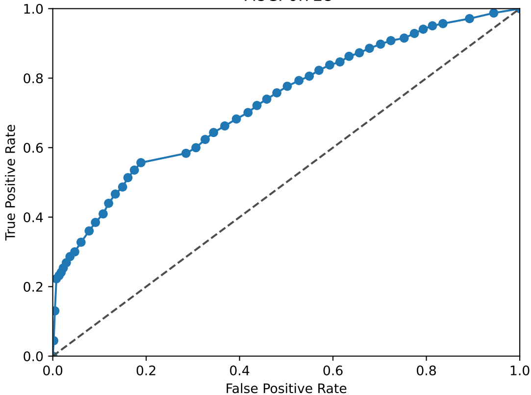
FOS ROC Curve AUC: 0.728
