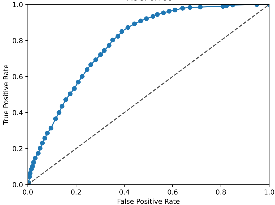
HSF2 ROC Curve AUC: 0.788
