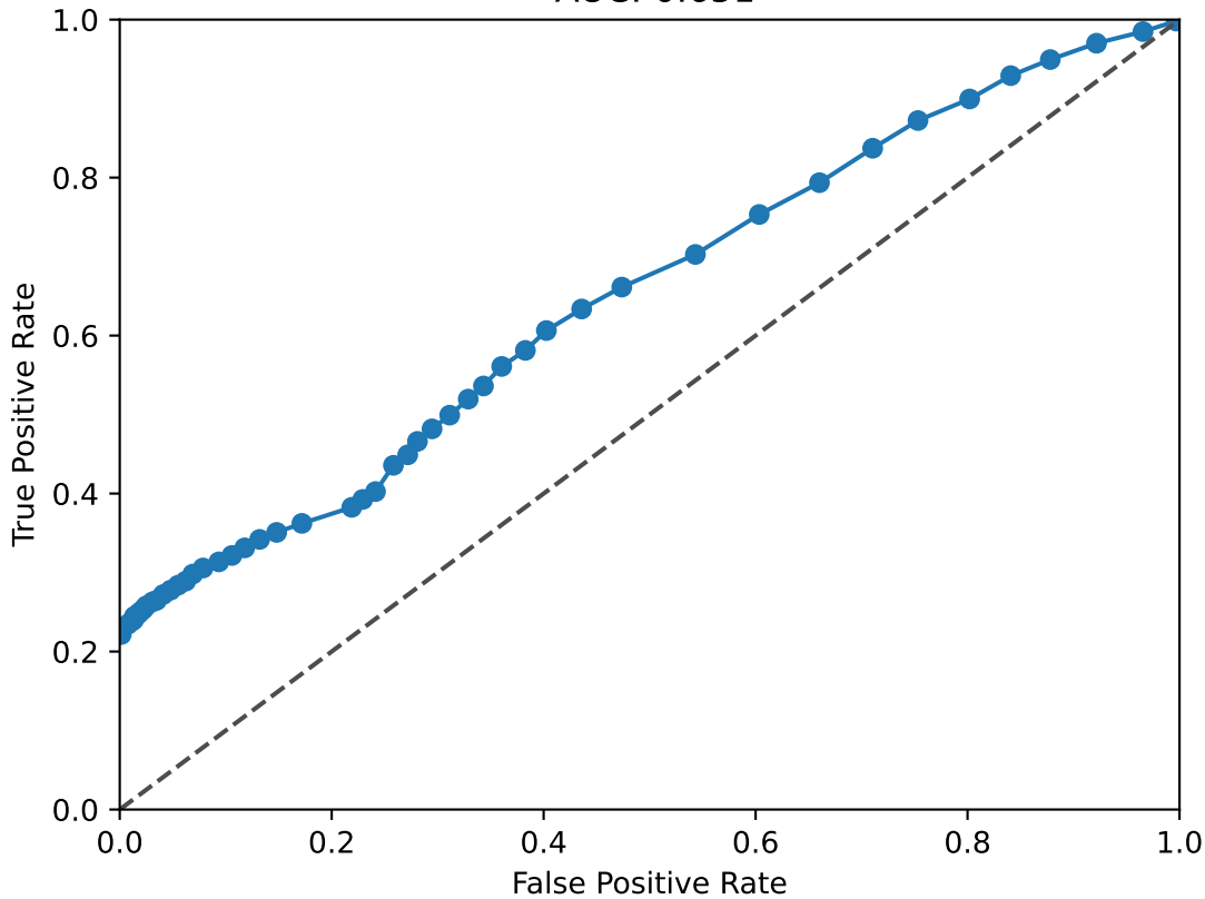
ICAM1 ROC Curve AUC: 0.651
