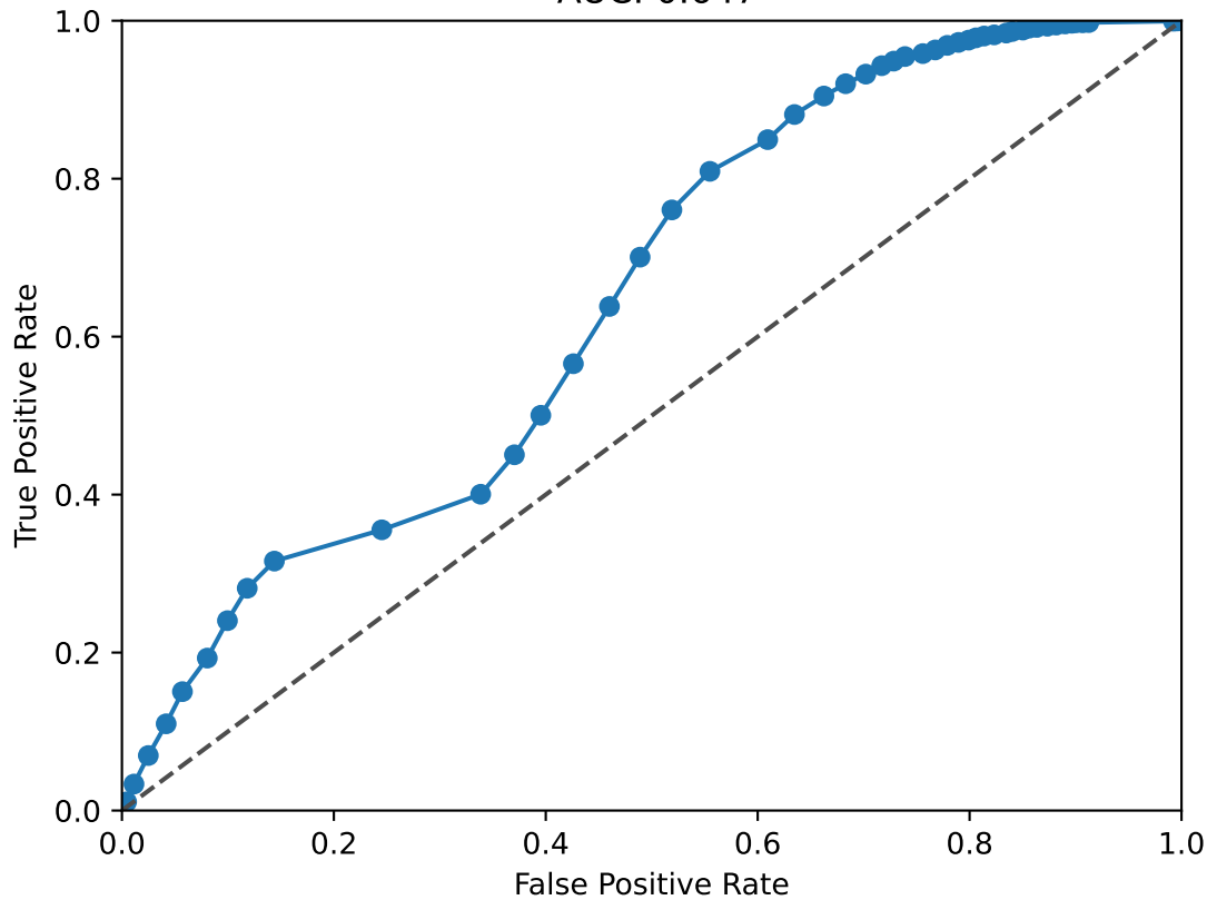
KMT2A ROC Curve AUC: 0.647
