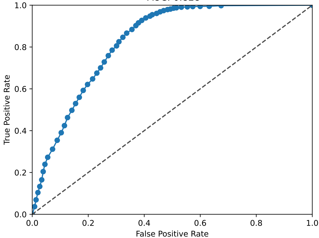
NCAM1 ROC Curve AUC: 0.828
