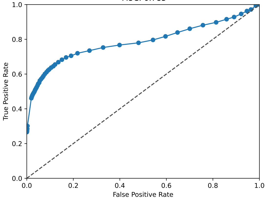
NFIX ROC Curve AUC: 0.785
