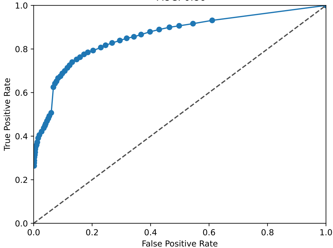
REST ROC Curve AUC: 0.86
