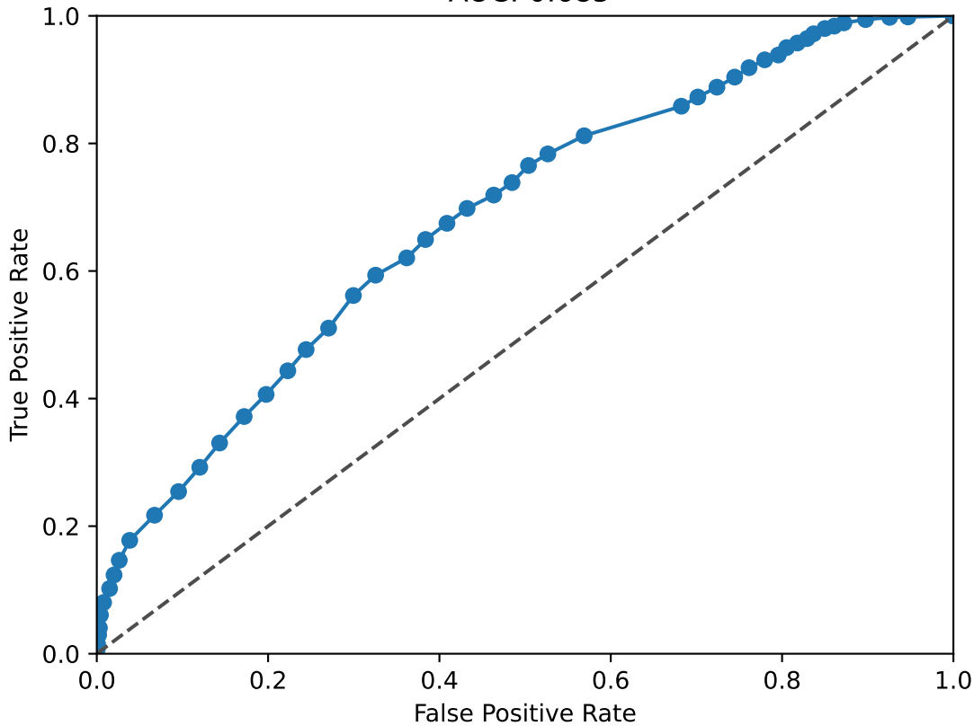
SIX4 ROC Curve AUC: 0.685
