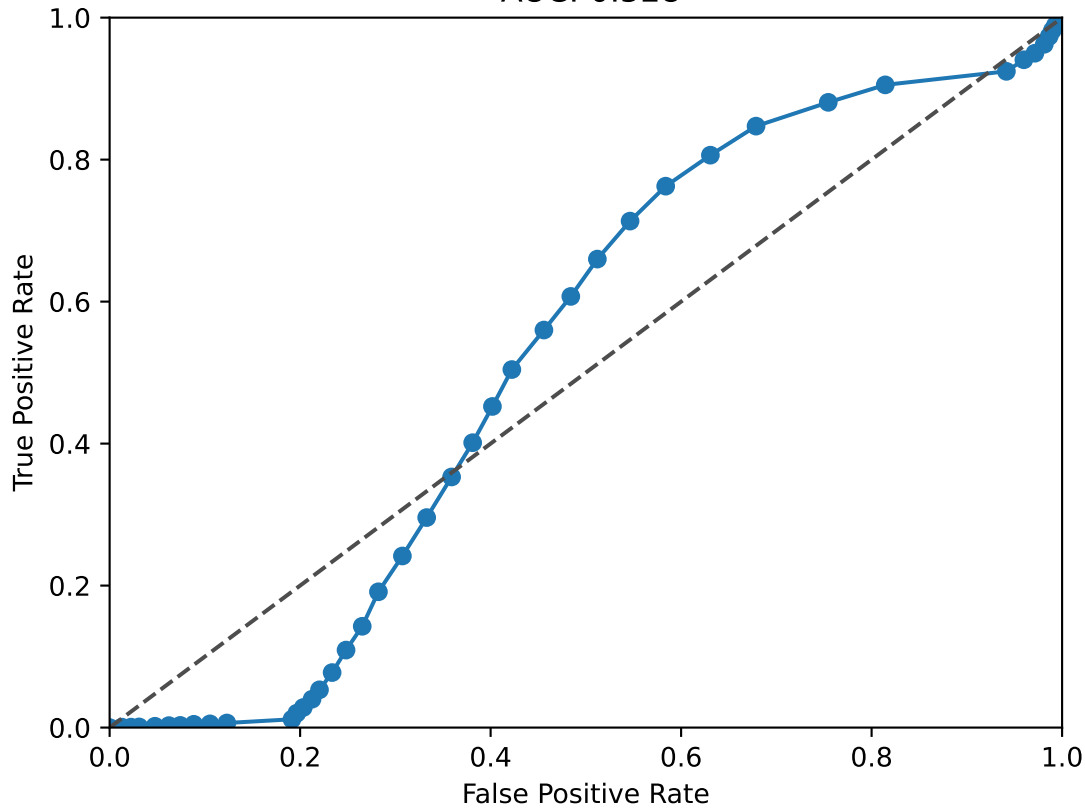
STAT2 ROC Curve AUC: 0.528
