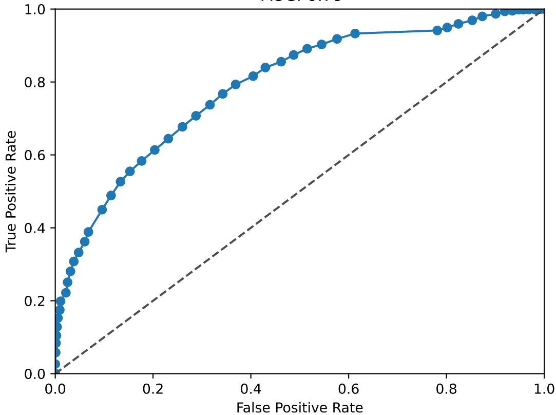
TBX15 ROC Curve AUC: 0.79
