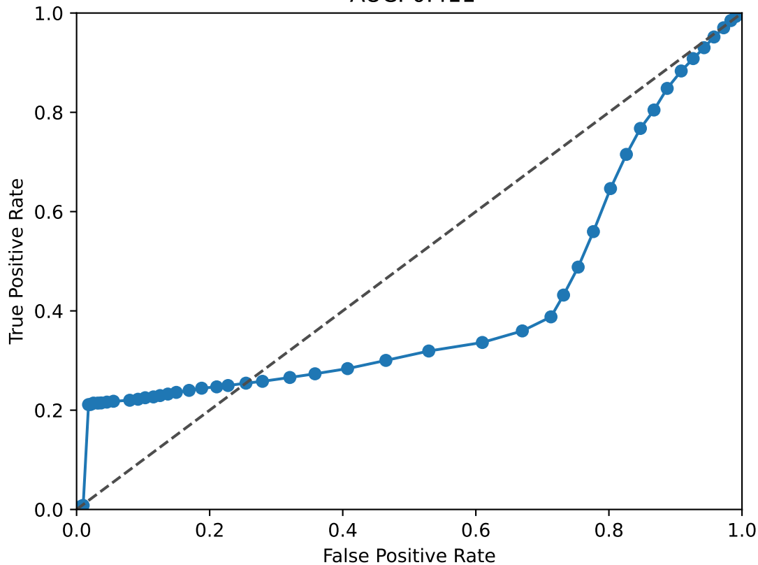
TCF7L1 ROC Curve AUC: 0.411
