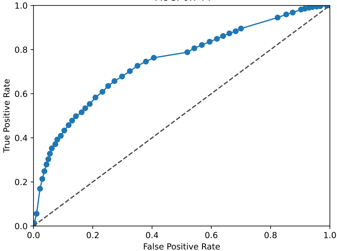
TEAD1 ROC Curve AUC: 0.744
