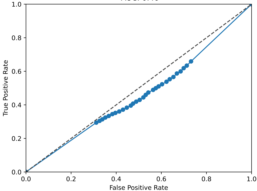
THR B ROC Curve AUC: 0.46
