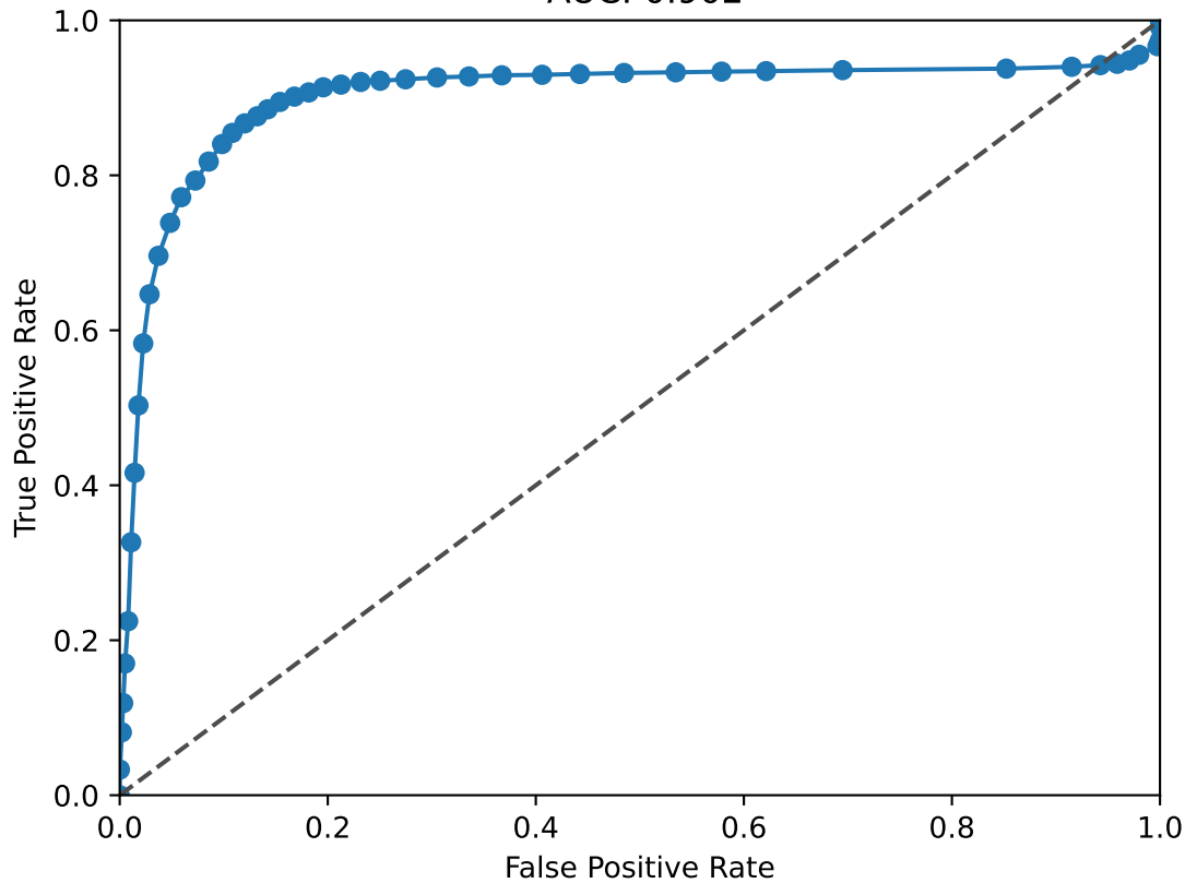
EGR1 ROC Curve AUC: 0.902
