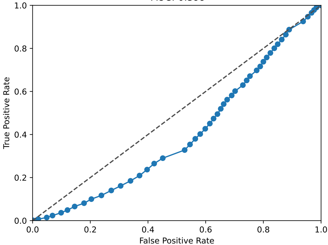
EPCAM ROC Curve AUC: 0.399
