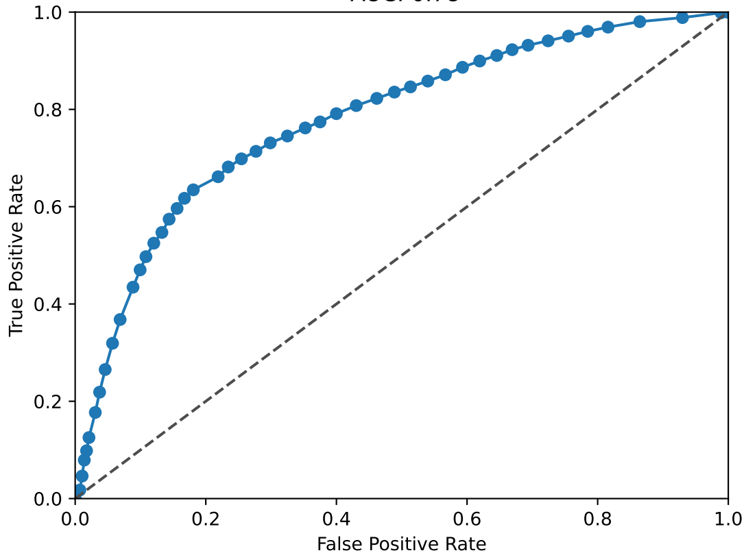
FOS ROC Curve AUC: 0.78
