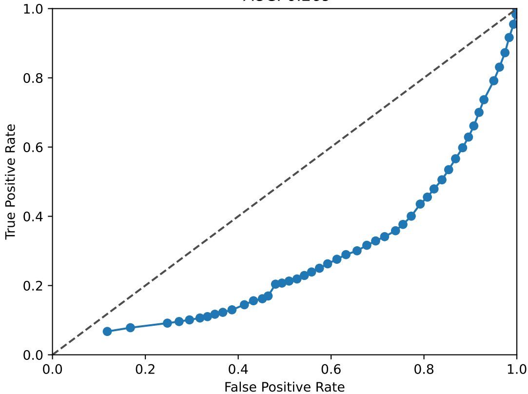
HES1 ROC Curve AUC: 0.269
