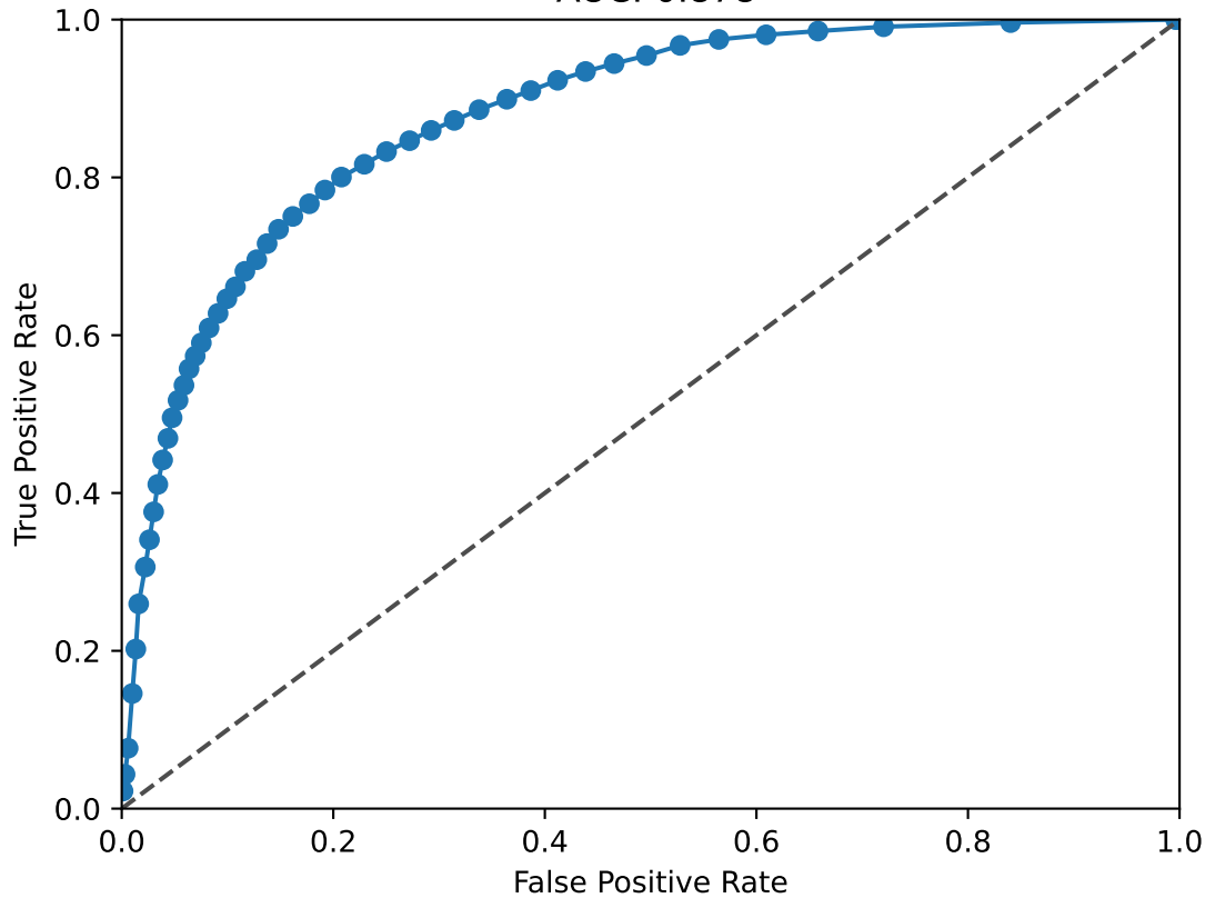
HSF2 ROC Curve AUC: 0.878
