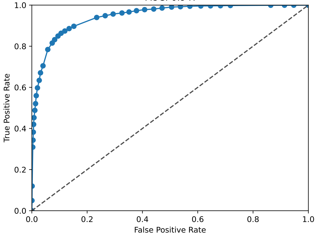
NFATC2 ROC Curve AUC: 0.947
