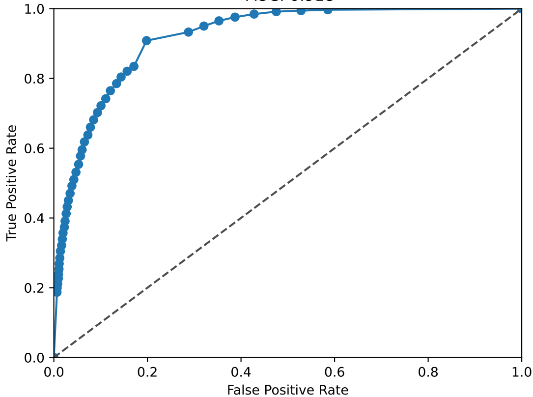
PROX1 ROC Curve AUC: 0.918
