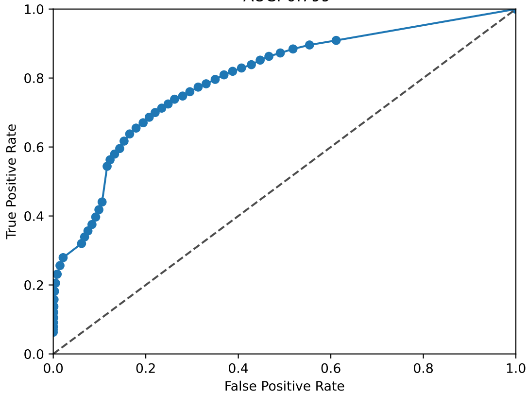
REST ROC Curve AUC: 0.799
