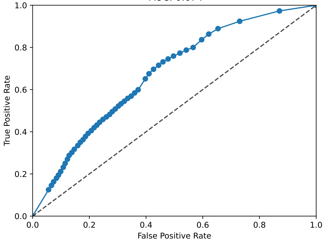
SIX1 ROC Curve AUC: 0.674
