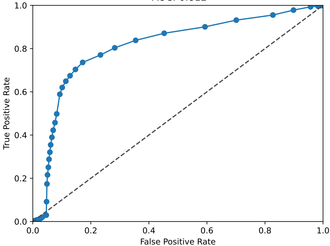
STAT2 ROC Curve AUC: 0.812
