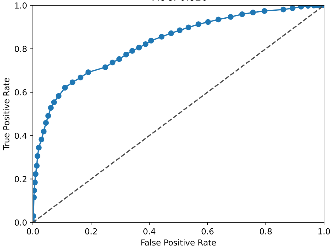
TBX15 ROC Curve AUC: 0.826
