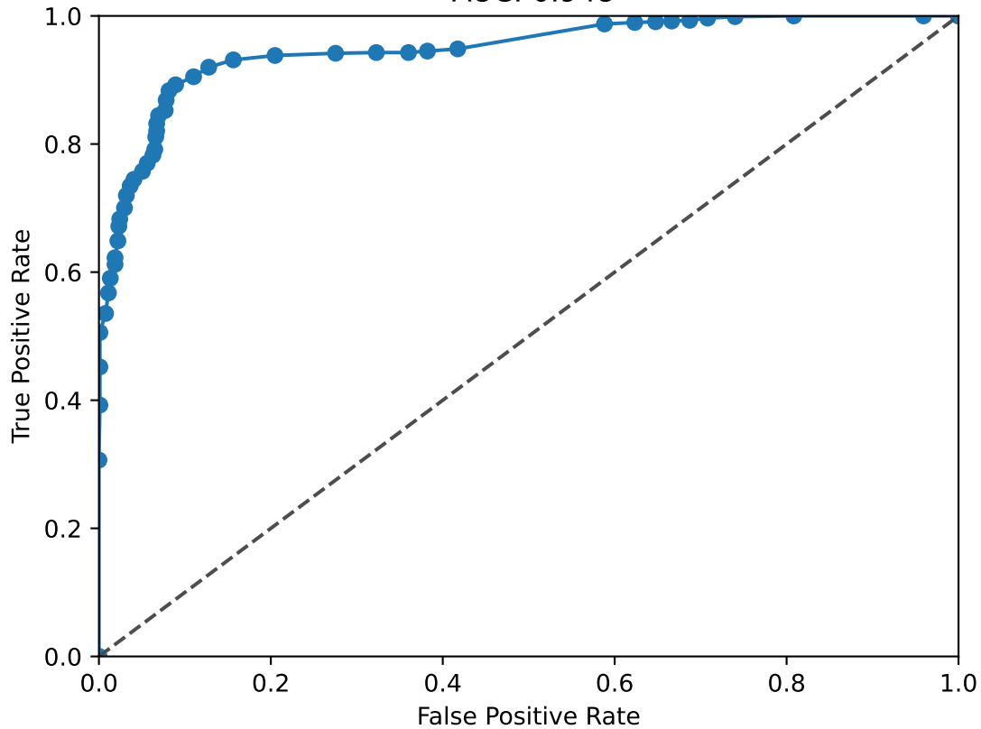
EGR1 ROC Curve AUC: 0.948
