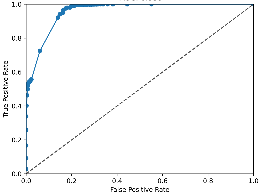
KMT2A ROC Curve AUC: 0.959
