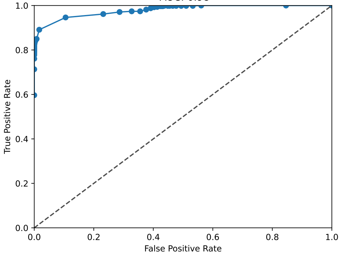
NFIX ROC Curve AUC: 0.98
