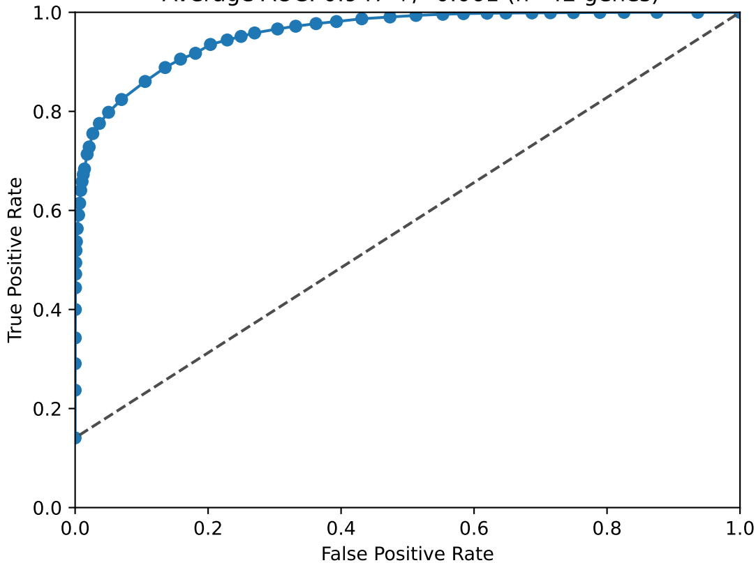
ROC Curve Data Average AUC: 0.947 \pm 0.061 (n=42 genes)
