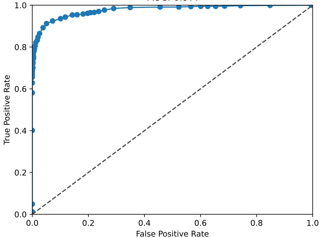
CUX2 ROC Curve AUC: 0.977
