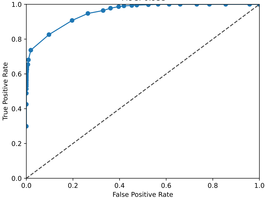
ICAM1 ROC Curve AUC: 0.953
