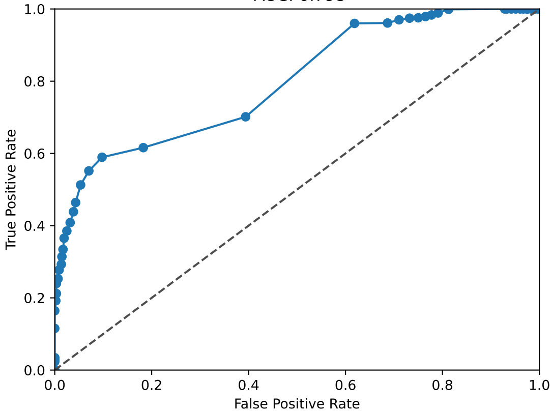
JUNB ROC Curve AUC: 0.798
