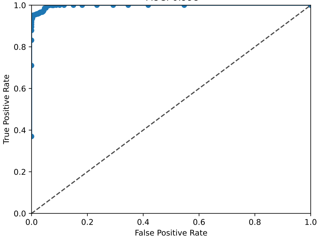
NFIB ROC Curve AUC: 0.998
