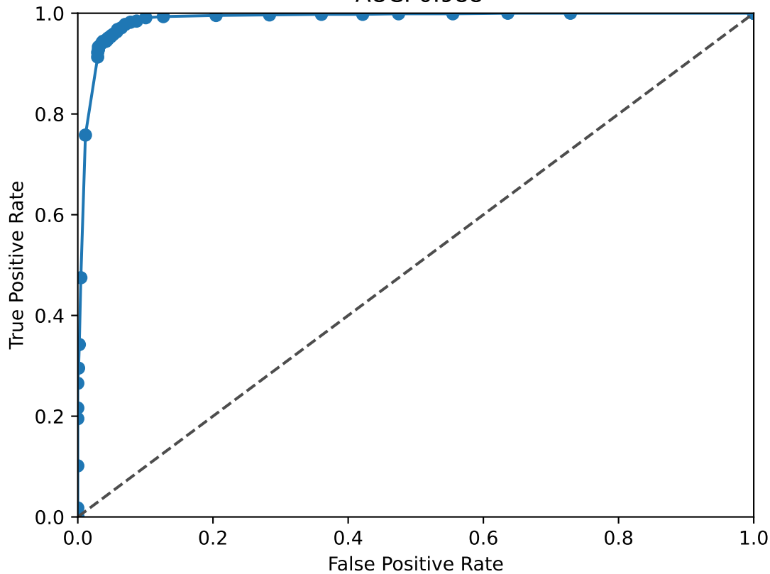
NFKB1 ROC Curve AUC: 0.988
