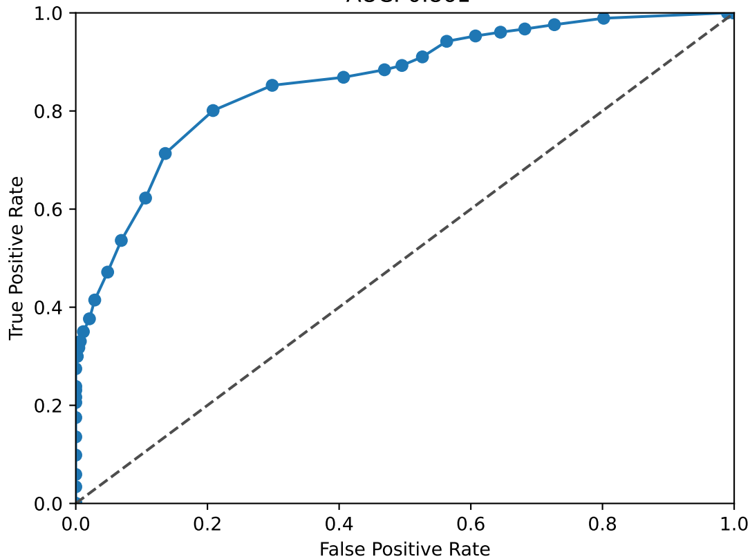
PBX1 ROC Curve AUC: 0.861
