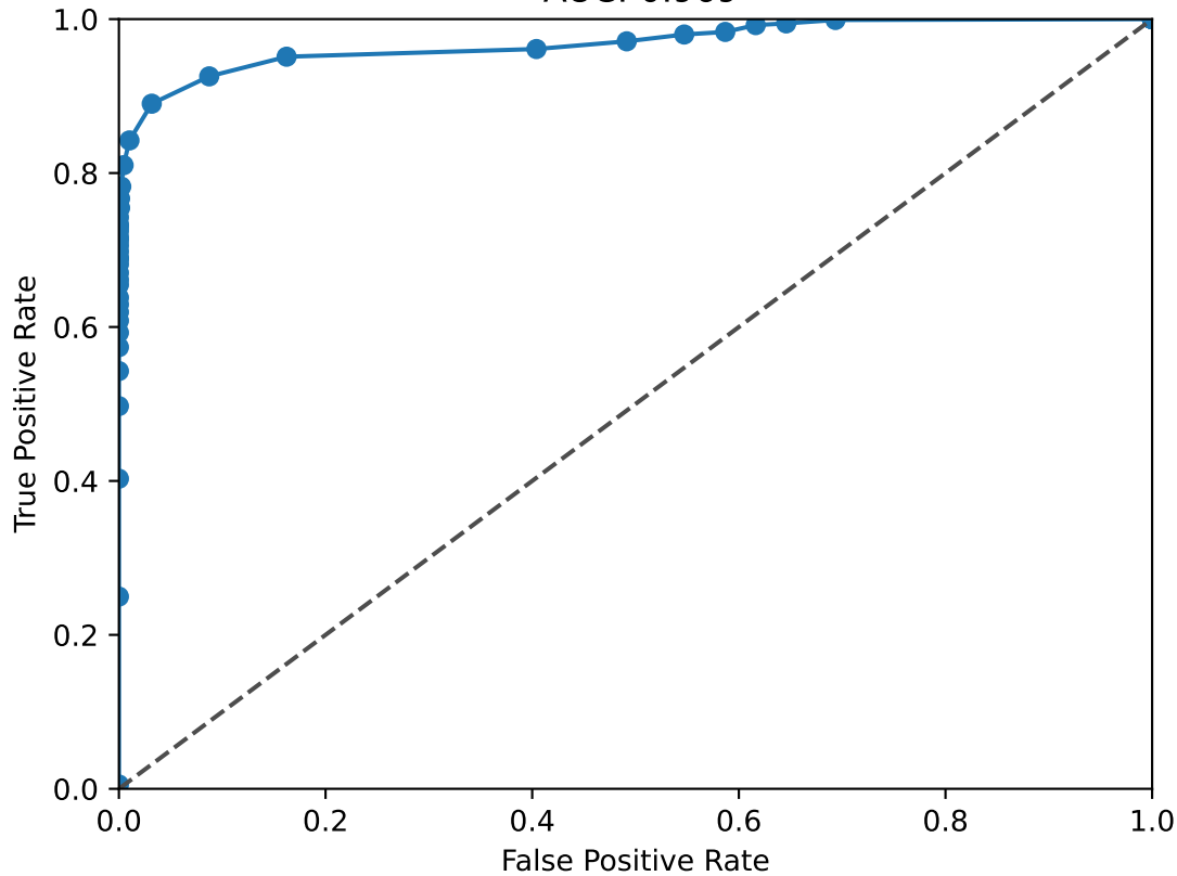
PROX1 ROC Curve AUC: 0.969
