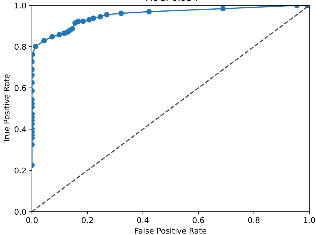
REST ROC Curve AUC: 0.954
