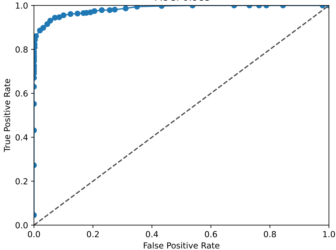
RORA_RORB ROC Curve AUC: 0.985
