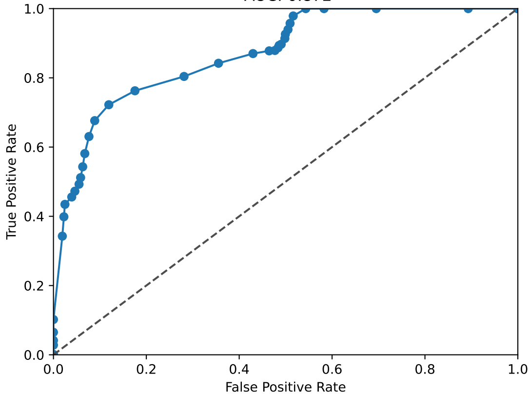
STAT2 ROC Curve AUC: 0.872
