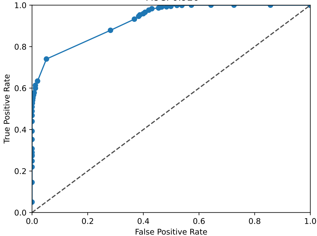
TCF7L1 ROC Curve AUC: 0.926
