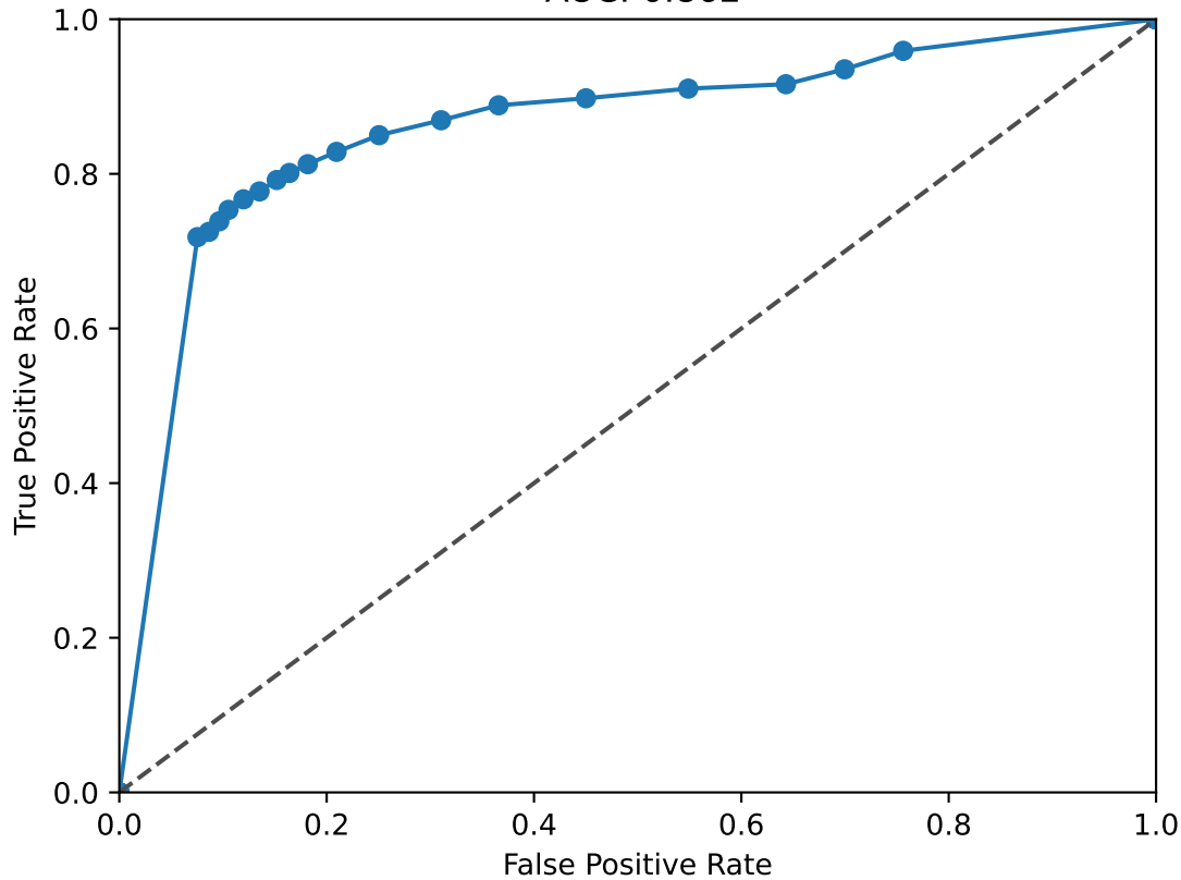
THR B ROC Curve AUC: 0.862
