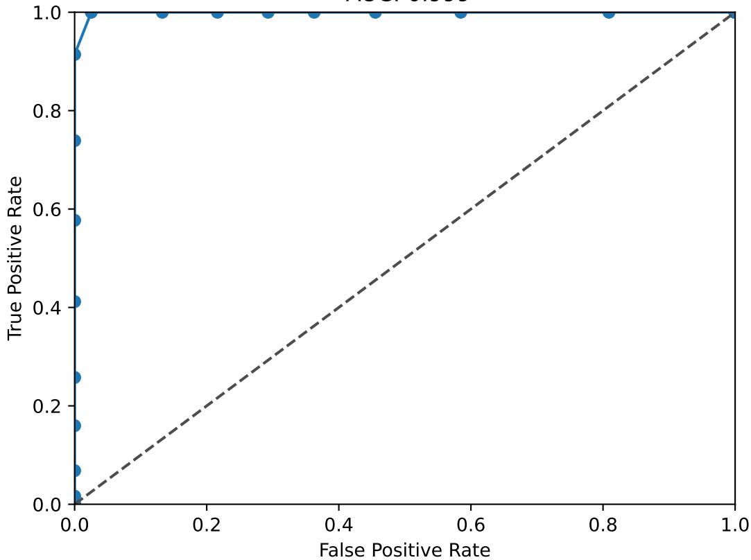
ZEB1 ROC Curve AUC: 0.999
