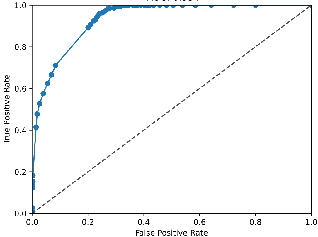
FOXO3 ROC Curve AUC: 0.934
