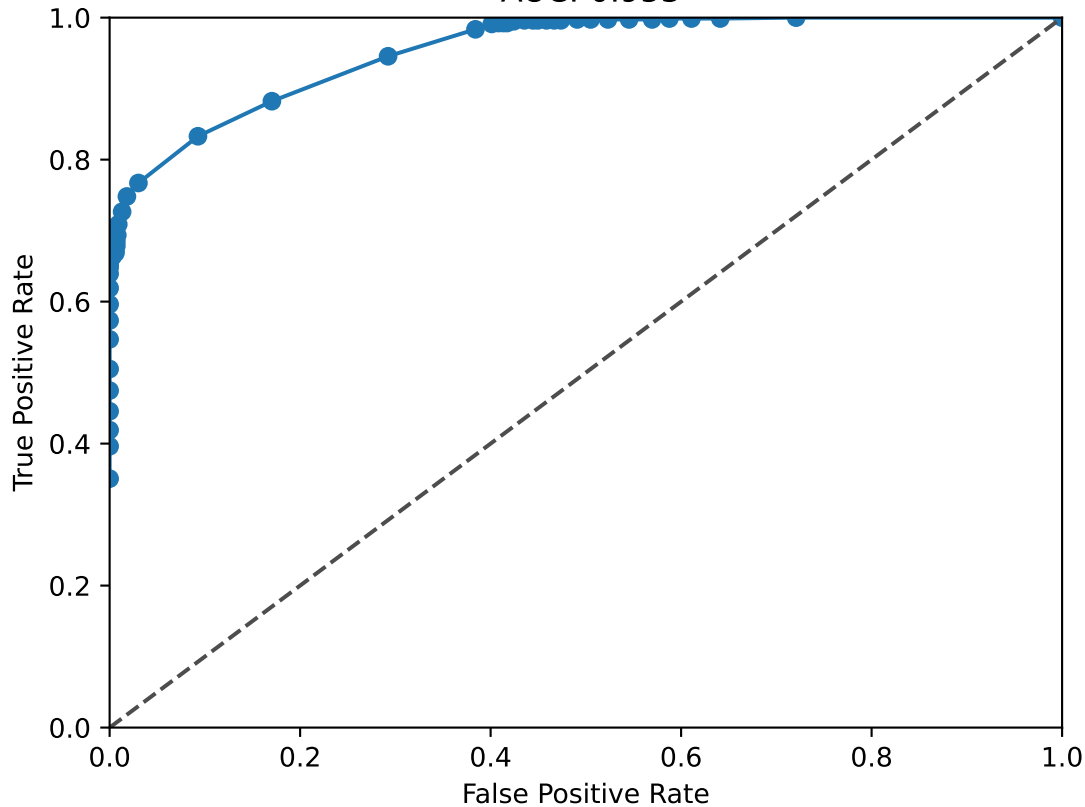
HES1 ROC Curve AUC: 0.953
