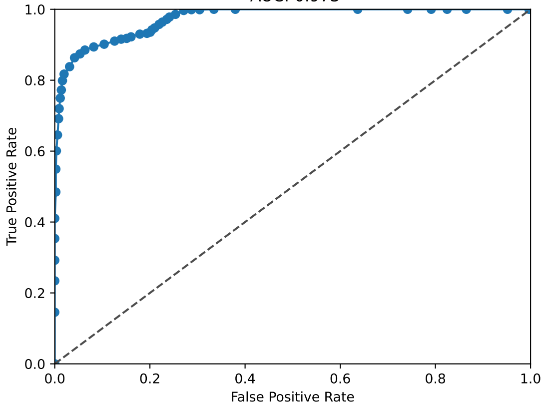
FOS ROC Curve AUC: 0.973
